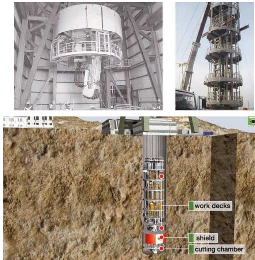
Cross Section of the Herrenknecht Shaft Sinker
